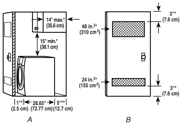
A. Side view - closet or confined area
